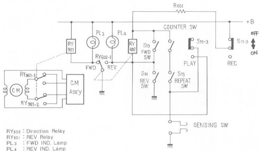
NOTE: The reversing relay RY 901 is located inside the capstan motor assembly.
