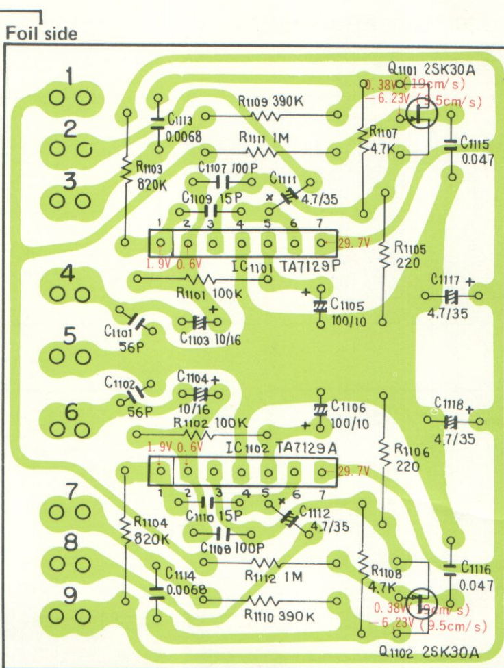
ON PLAYBACK AMPLIFIER ASSEMBLY (RWF-069)
